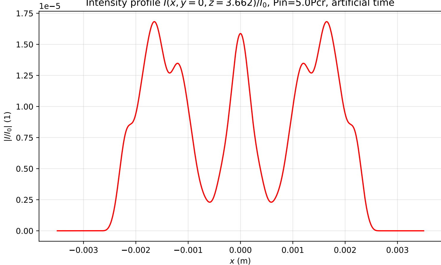
Intensity profile I(x, y = 0, z = 3.662)/I_0 , P_{in}=5.0P_{cr} , artificial time
